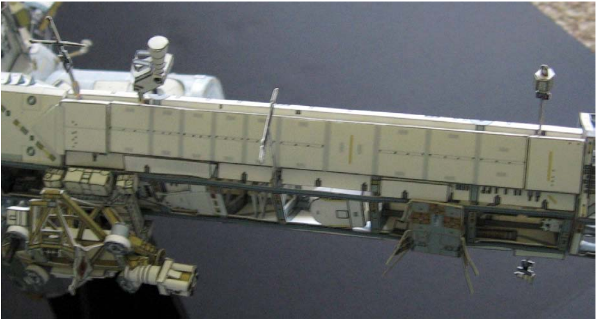
Location of Antennas on Starboard truss section
